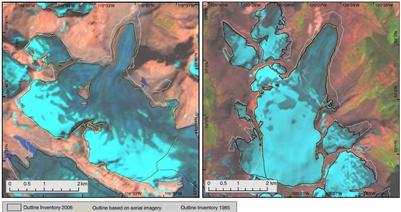
Fig. 4. Deviation of glacier outlines digitized manually from high resolution aerial photography (Matt Beedle, pers comm., 2007) and derived from Landsat TM data using our automated approach; left: Peyto Glacier in the southern Rocky Mountains, right: Castle Creek Glacier in the southern Interior Ranges; the arrows indicate problematic areas: A: Drainage basin delineation, B: Different interpretation of snow cover, C: Internal rocks, D: Debris-cover.
