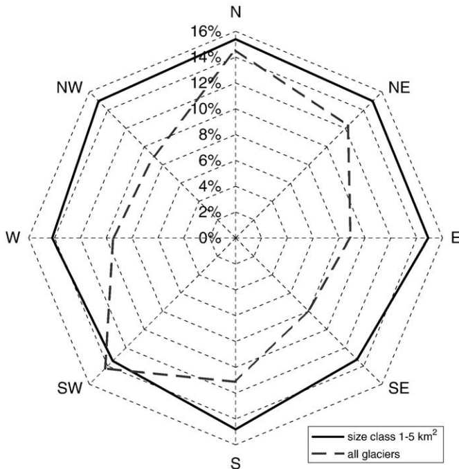
Fig. 9. Diagram showing area loss versus aspect for the whole study area.
