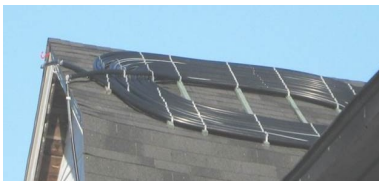
Coiled PEX pipe warms water
