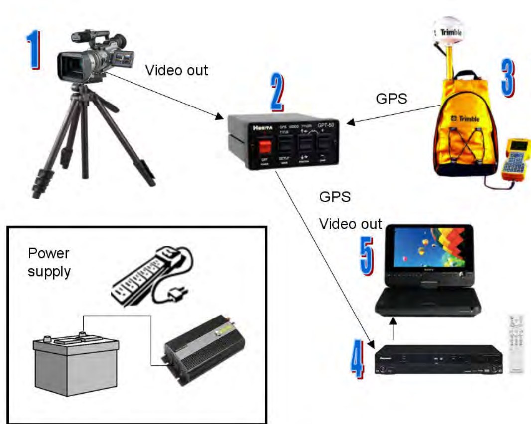
Figure 1: Shoreline video setup. 1) Digital video camera, 2) GPS stamper unit, 3) GPS data logger and receiver, 4) Digital video recorder, 5) Digital video player
